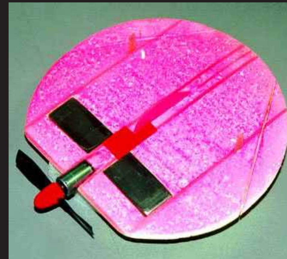
MITE, Naval Research Lab., USA
